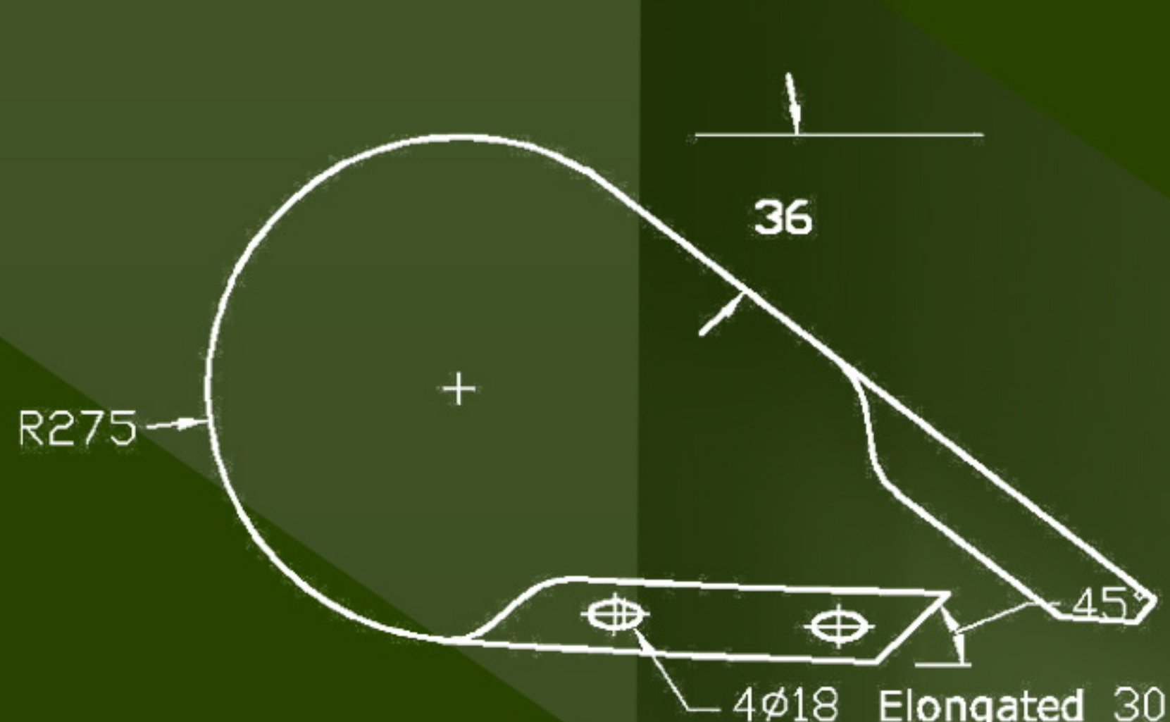
⊕ TERMINAL END BULLNOSE
