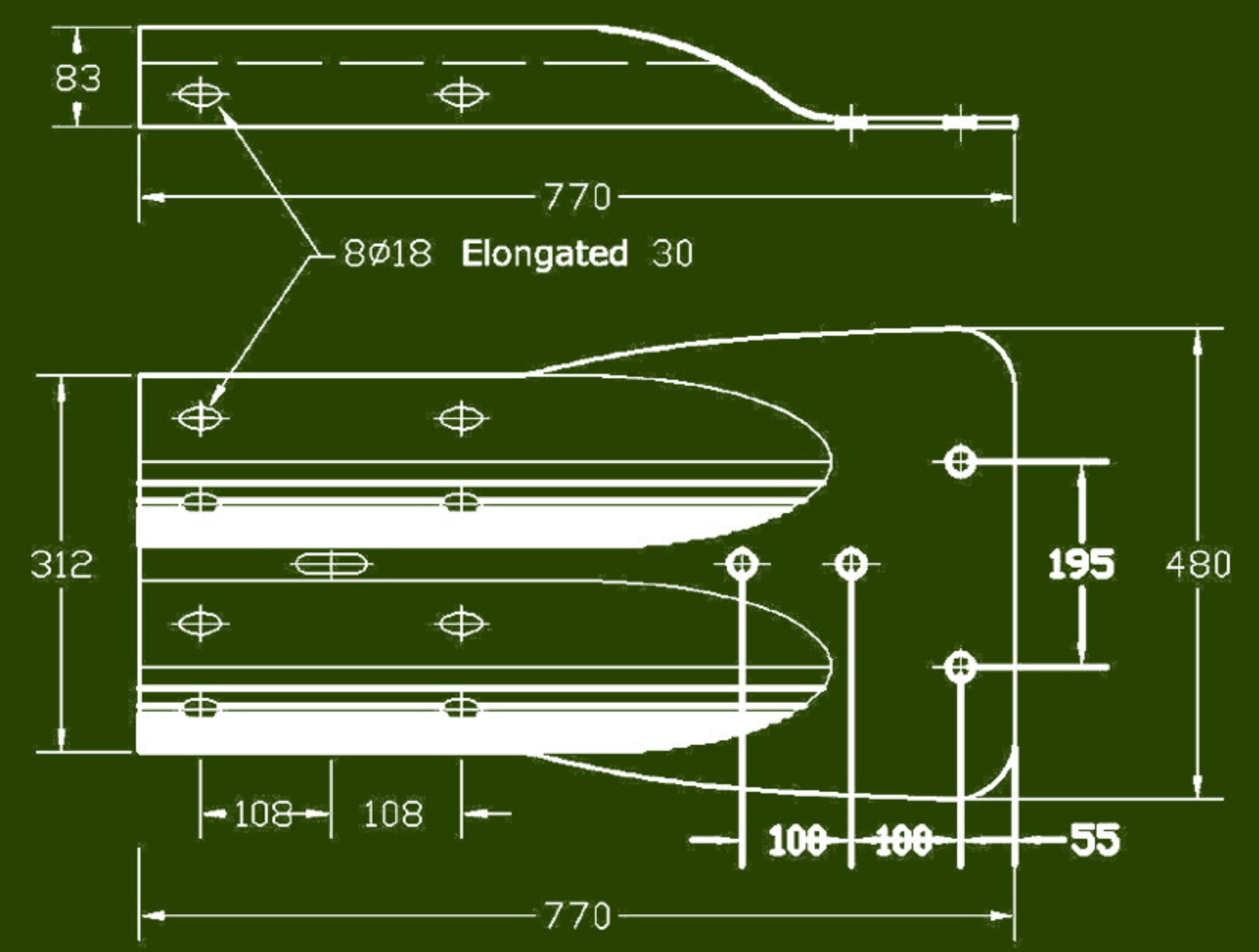
⊕ TERMINAL END SHOE
